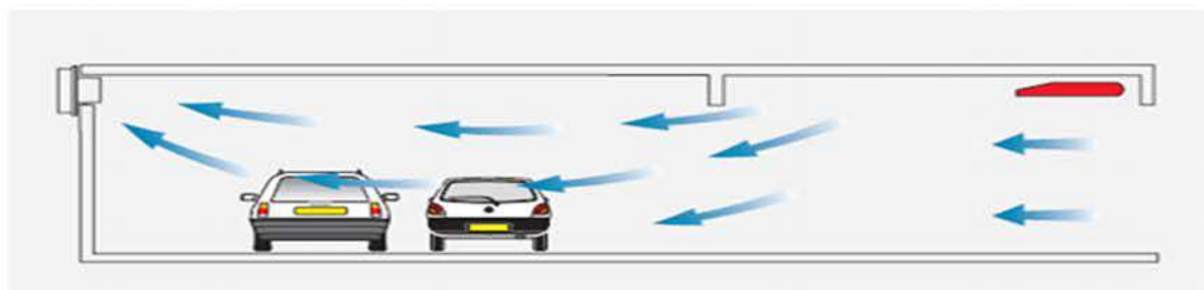
Air turbulence created by the downstands when using a typical impulse fan
